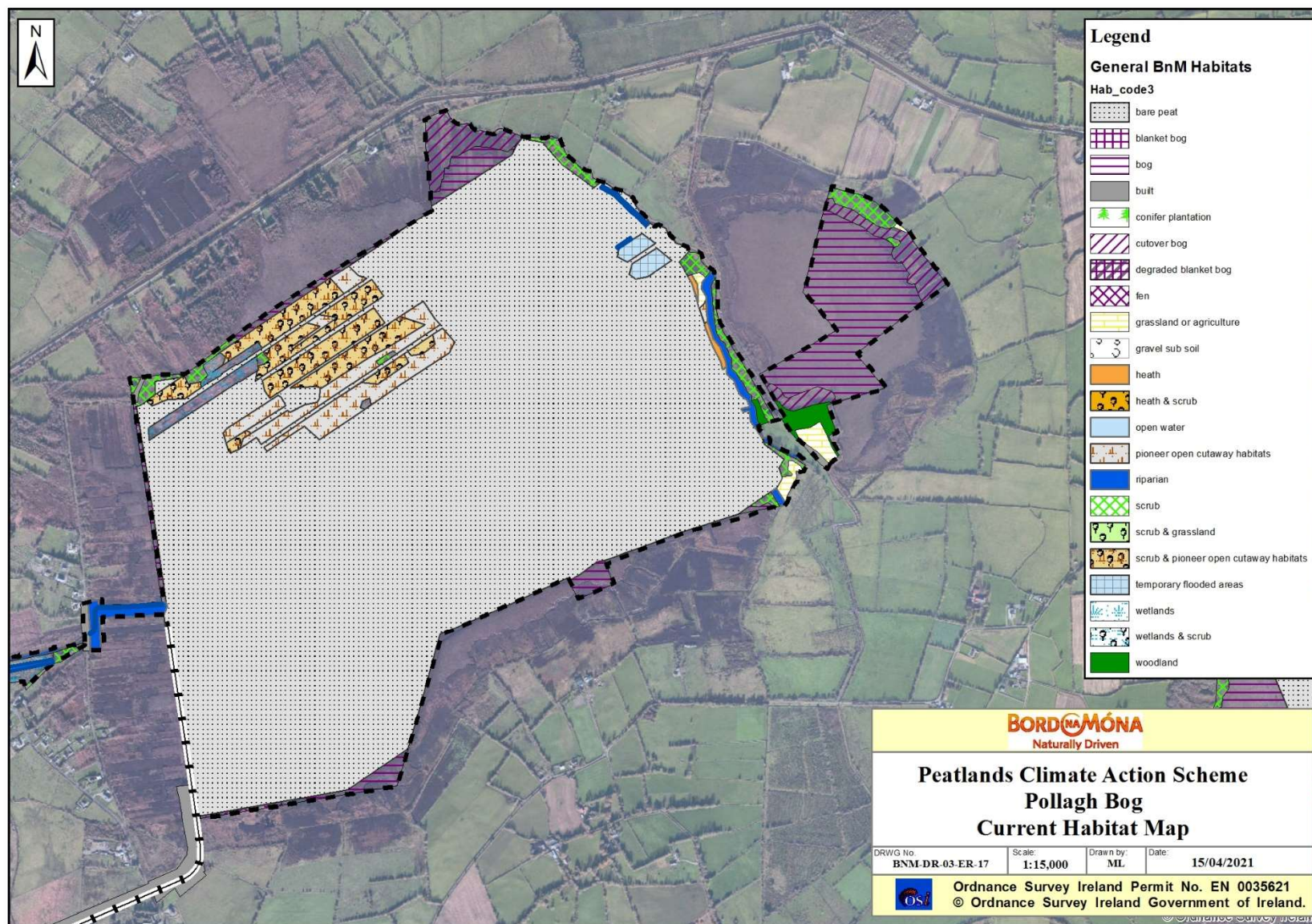
Figure 3.5. Habitat map of Pollagh Bog showing Bord na Móña habitat categorisation.
