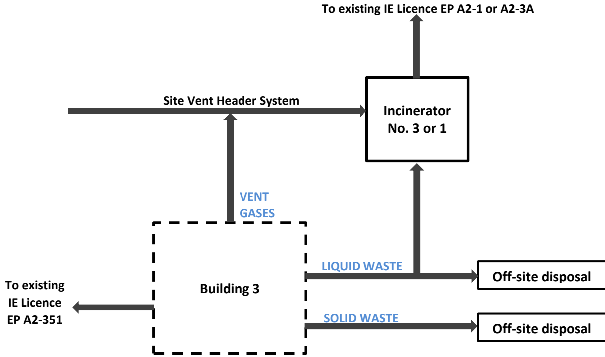
Figure 2.1 Project MARK Associated Environmental Emissions (Building 3)
