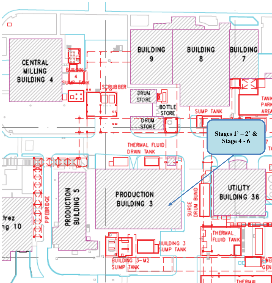
Figure 1.1 Site Layout and Location of Proposed Process for Project MARK
