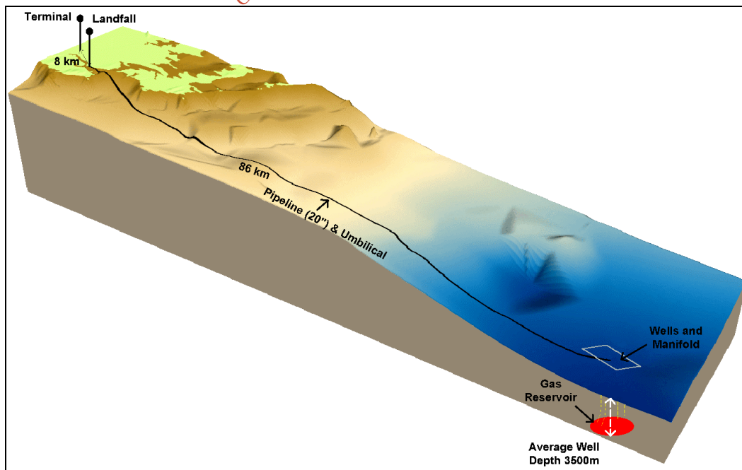
Figure 3 Corrib Development
