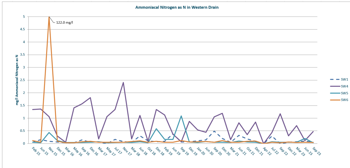
Graph 7.4 - Ammoniacal Nitrogen Trends in Surface Water
