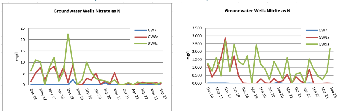
Graph 7.3 – Nitrate and Nitrite in GW7, GW8a and GW9a
