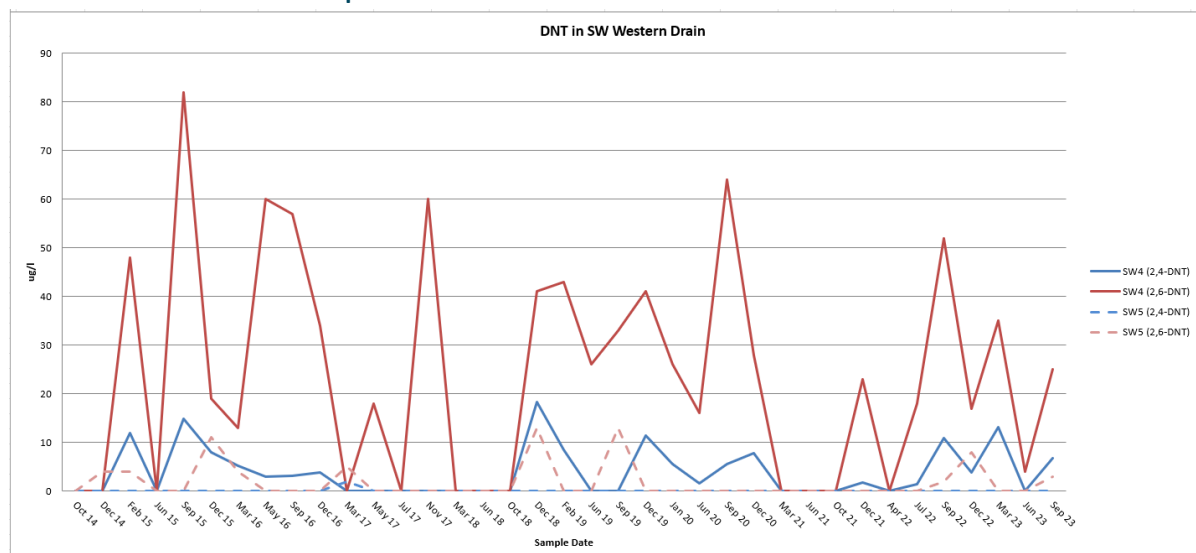
Graph 7.5 - Nitrotoluenes Trends in the Western Drain
