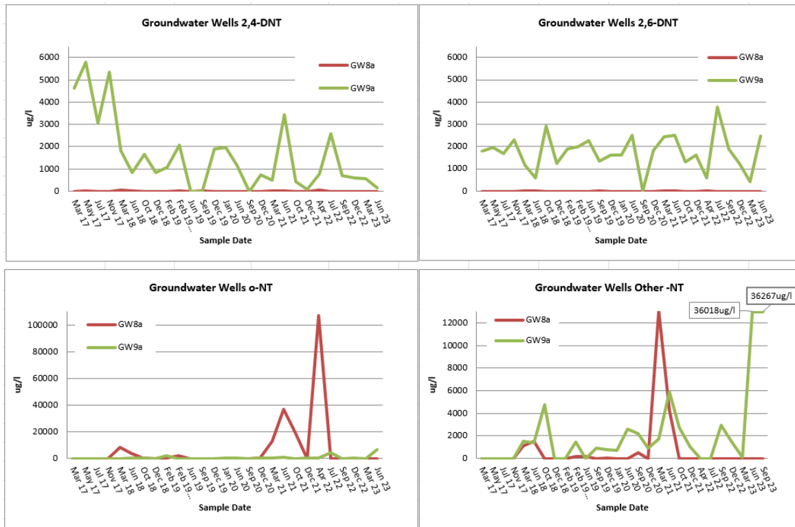
Graph 7.1 – Nitrotoluenes (ug/l) in Groundwater Wells GW8A and GW9A
